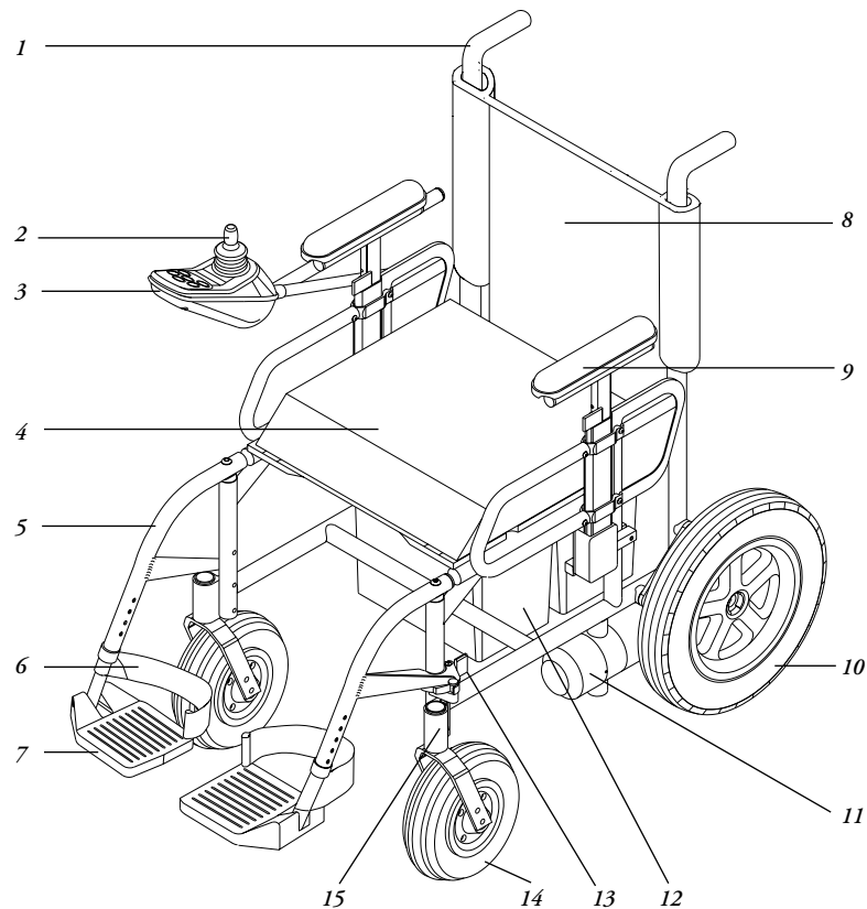
Quickie V-100 (Rigid frame)
