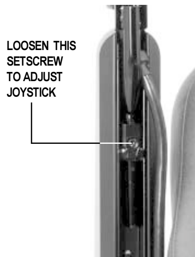
Figure 16. Joystick Extension
